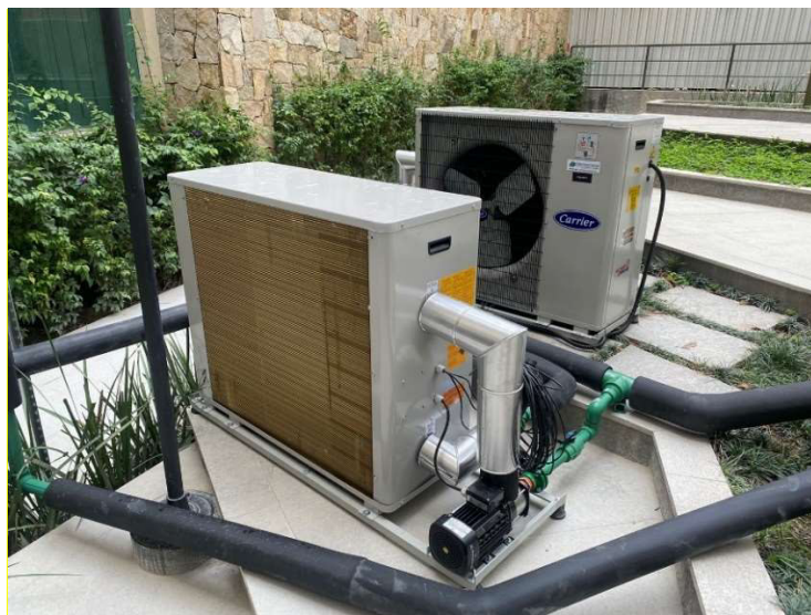
Figura 1- Chiller RM
